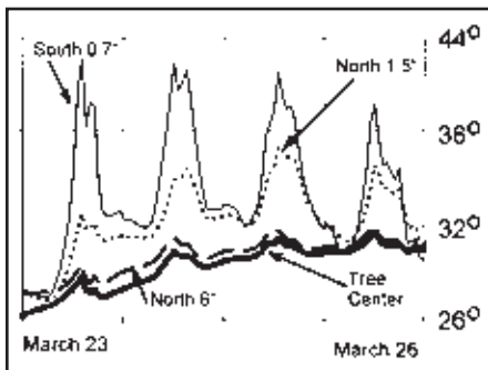
Figure 3: Variation in tree trunk temperature at different depths and aspects on four days in March, 2006.
