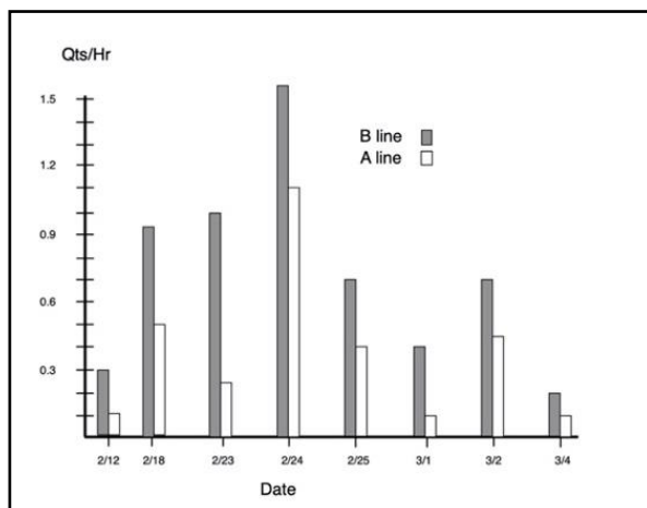
Figure 7 – Controlled study of walnut sap flow Line A – without vacuum, Line B- with vacuum (Rechlin, 2921).
