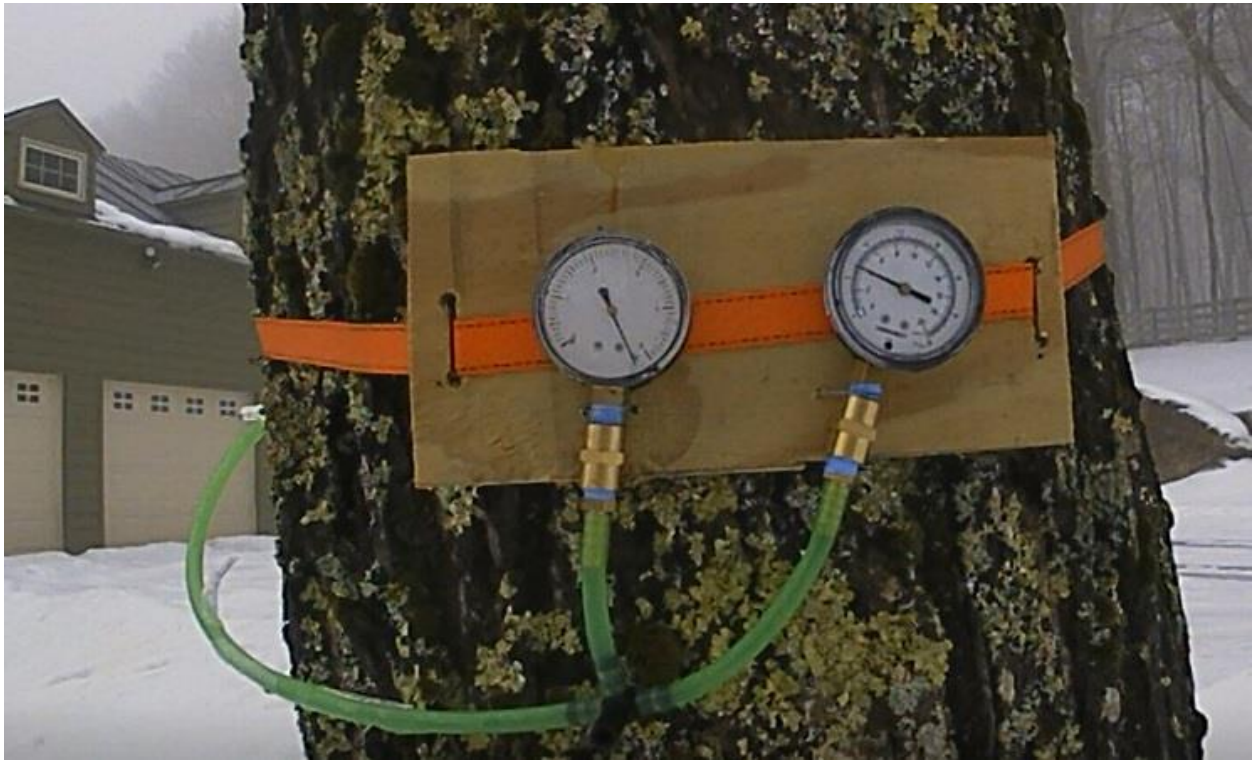
Figure 4 – Pressure gauges on a tapped walnut tree, the left, more sensitive gauge is pegged at 5 pounds and the right gauge reads 4 pounds.
