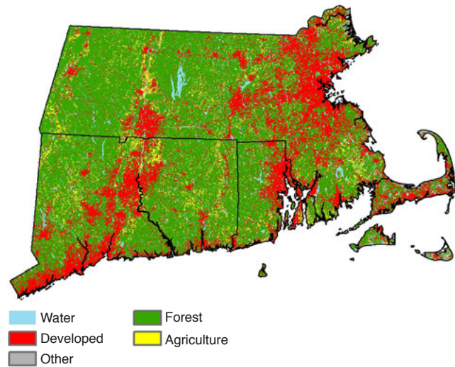
Figure 7. —Land cover, Southern New England, 2010 (Jin et al. 2013).
