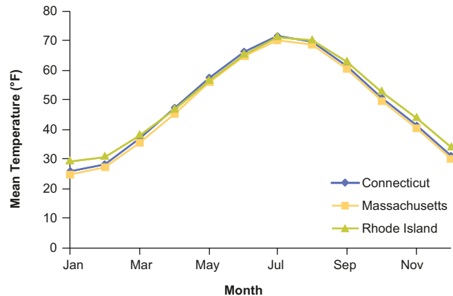
Figure 2. —Mean monthly temperatures for Connecticut, Massachusetts, and Rhode Island (NOAA, n.d.a.).
