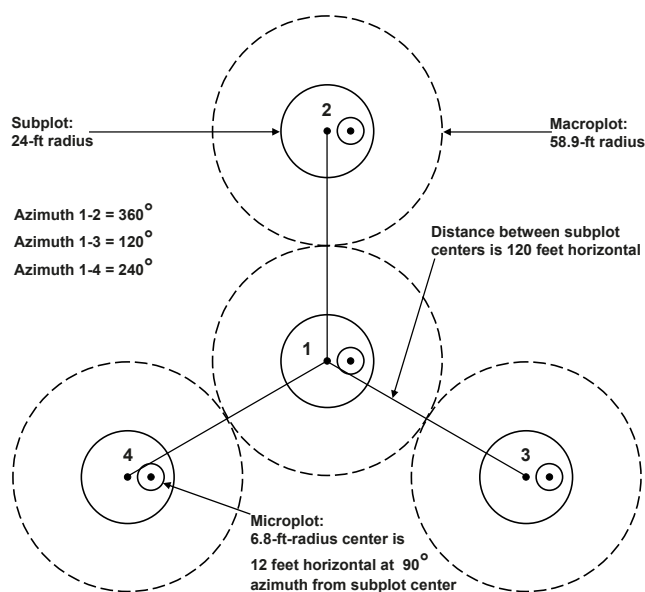
Figure 1. —U.S. Forest Service, Forest Inventory and Analysis plot layout (adapted from Bechtold and Patterson 2005). Macroplots are not used in Southern New England.
