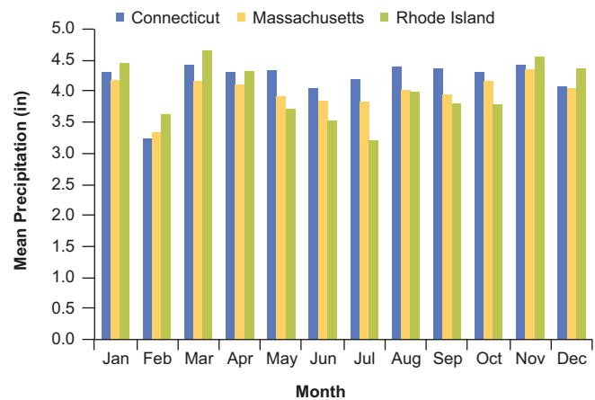
Figure 3. —Mean monthly precipitation for Connecticut, Massachusetts, and Rhode Island (NOAA, n.d.b.).
