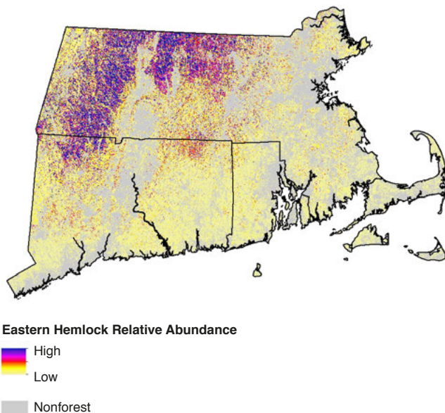
Figure 37. —Relative abundance of eastern hemlock, Southern New England, 2012.
