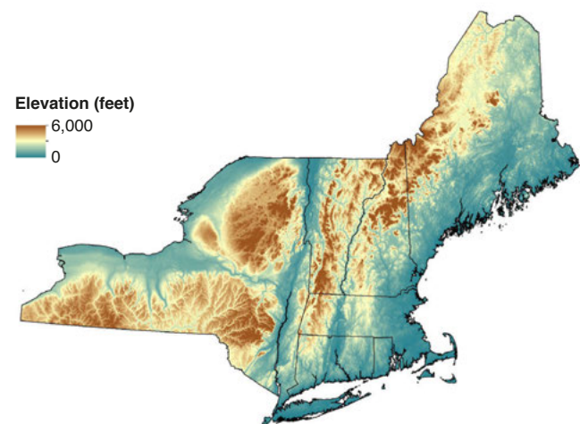
Figure 4. —Topography of the northeastern United States (USGS 2014).
