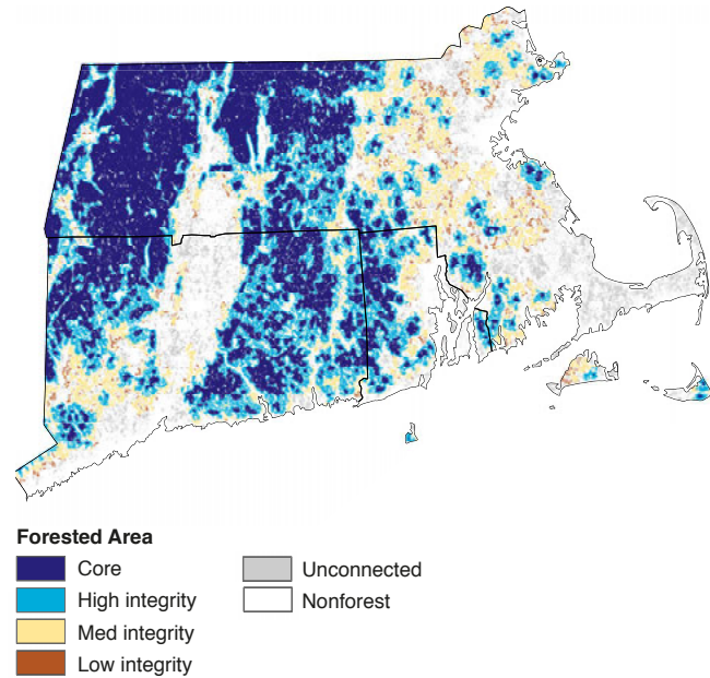
Figure 11. —Forest land by spatial integrity index (SII) at the 250 m scale, 2009. Processing note: Map was produced by calculating spatial integrity index for every forest pixel in the 250 m 2009 FIA modeled forest/nonforest dataset (Wilson et al. 2012). See text for explanation of special integrity index.
