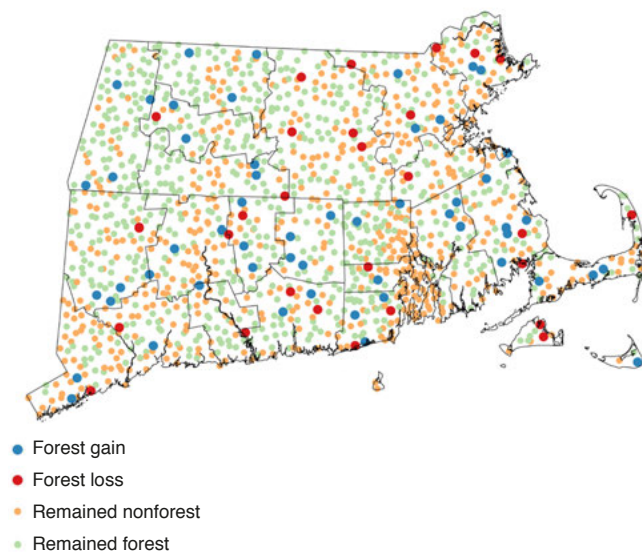
Figure 10. —Distribution of remeasured inventory plots showing forest gains and losses, as well as plots that were unchanged, Southern New England, 2007 to 2012. (Plot locations are approximate.)
