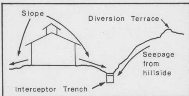
Figure 1. Surface drainage.
