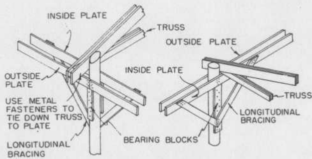
PLATE DETAIL
