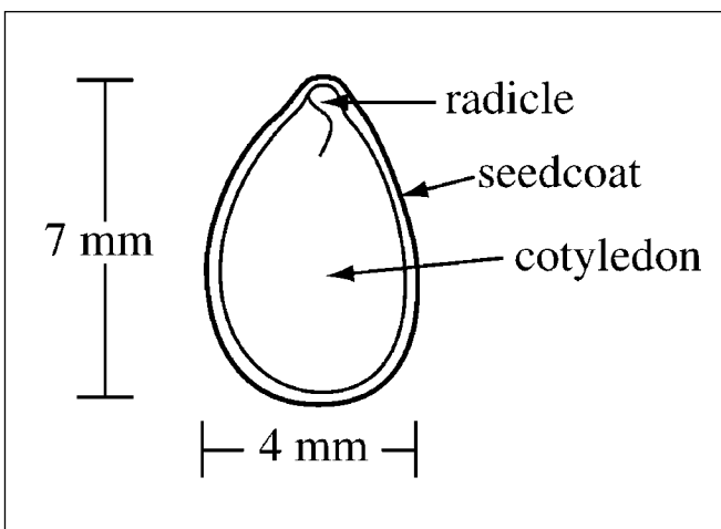
Figure 2 — Psoralea arborescens var. simplifolius , California dalea: longitudinal section through a seed.
