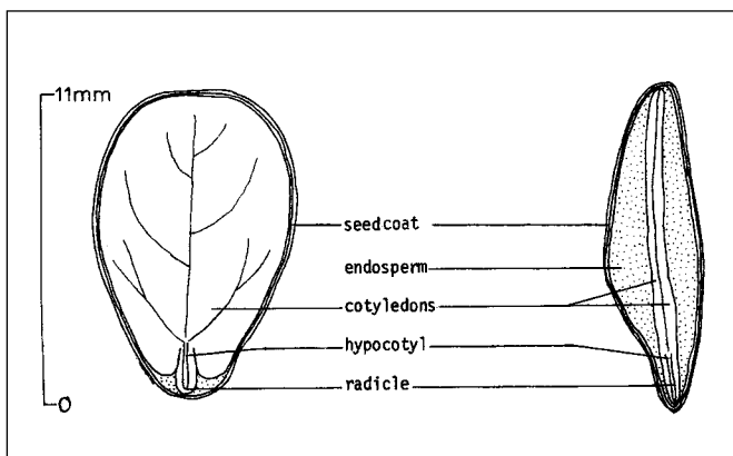
Figure 2 — Ceratonia siliqua , carob: longitudinal sections through a seed.
