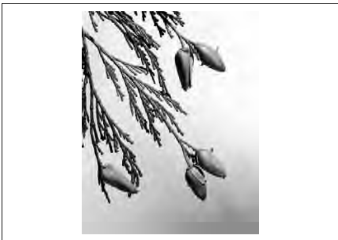
Figure 1 — Calocedrus decurrens , incense-cedar: cones hang singly from branch tips well-dispersed over the crown and contain up to 4 seeds each.
