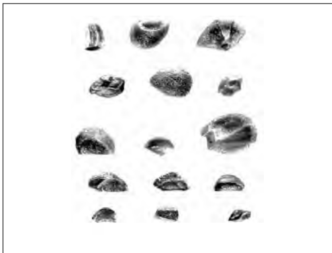
Figure 1 — Eucalyptus , eucalyptus: seeds (from left to right) of E. camaldulensis , river redgum eucalyptus; E. delegatensis , alpine-ash eucalyptus; and E. fastigata , brown-barrel eucalyptus ( top ). E. grandis , rosegum eucalyptus; E. microcorys , tallowwood eucalyptus; E. nitens , shining eucalyptus ( second row ). E. obliqua , messmate stringybark eucalyptus; E. paniculata , gray ironbark eucalyptus; and E. pilularis , blackbutt eucalyptus ( third row ). E. regnans , mountain-ash eucalyptus, E. robusta , robusta eucalyptus; and E. rudis , desert eucalyptus ( fourth row ). E. saligna , saligna eucalyptus; E. sideroxylon , red ironbark eucalyptus; and E. viminalis , manna eucalyptus ( bottom row ).
